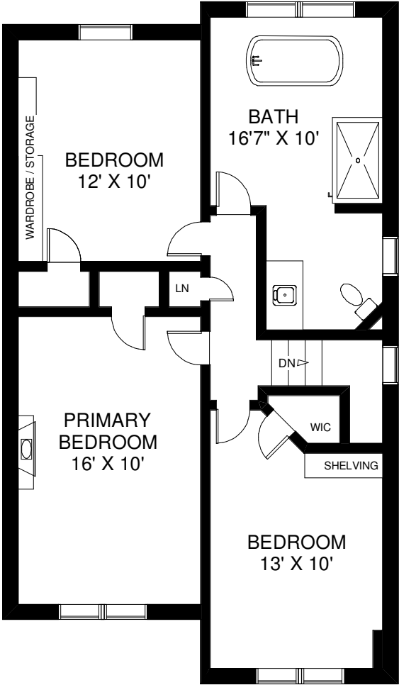
SECOND FLOOR
