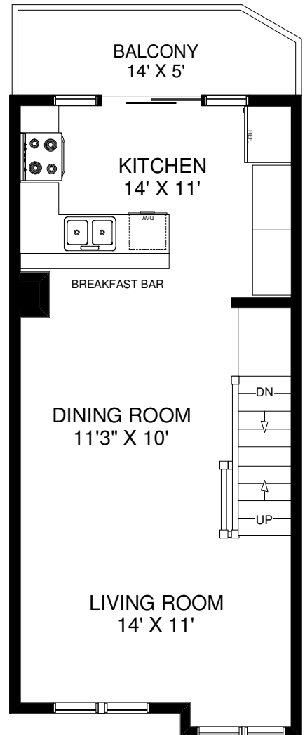
MAIN FLOOR
