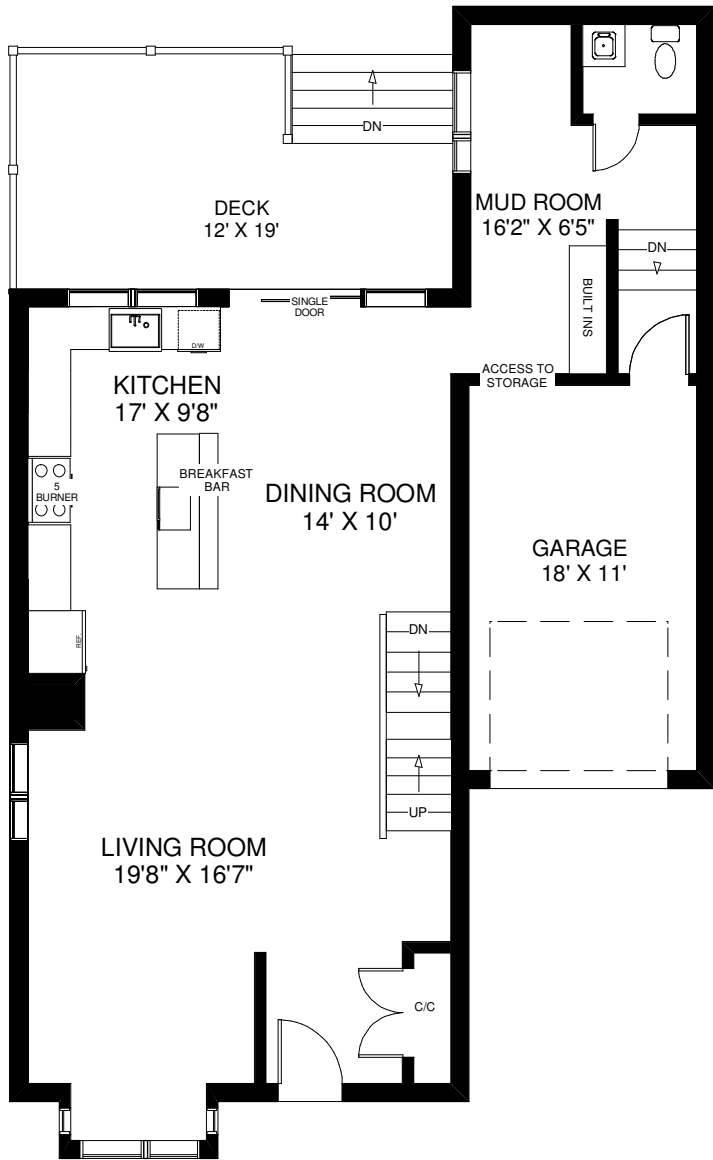
MAIN FLOOR
