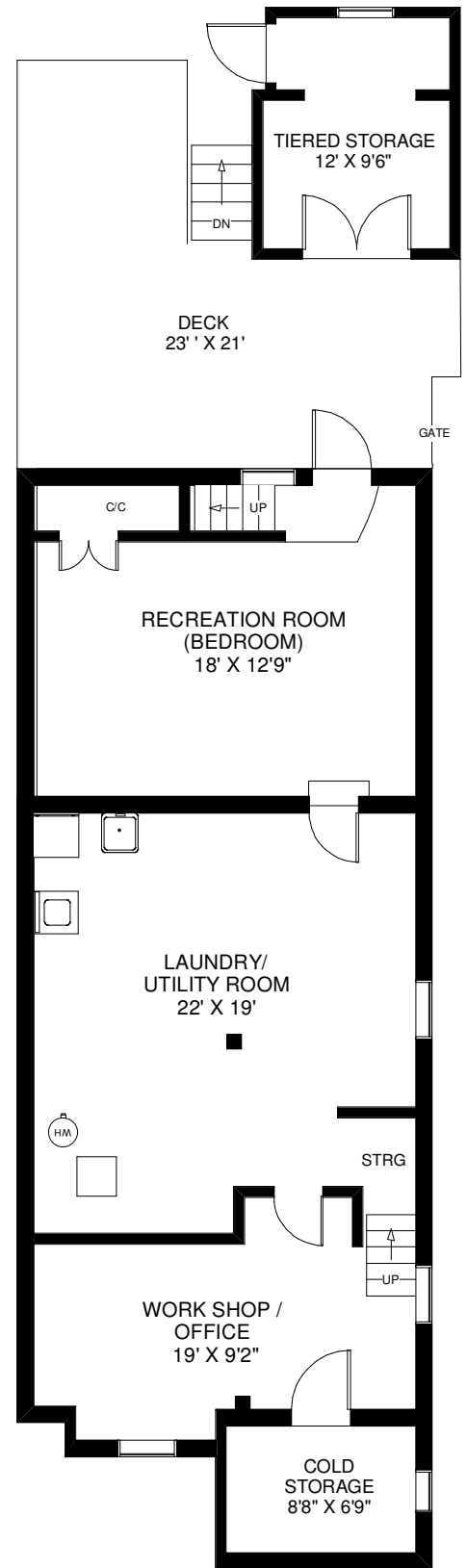
LOWER FLOOR
