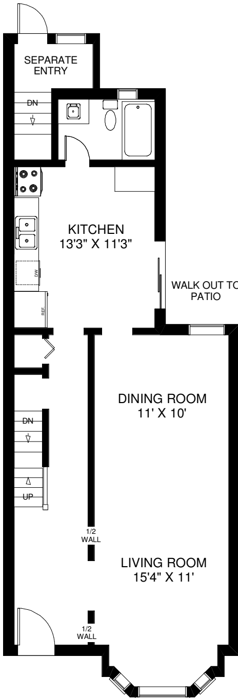
MAIN FLOOR
