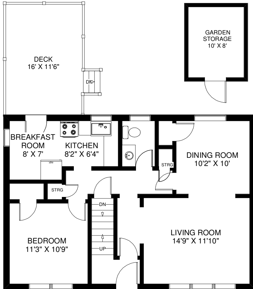
MAIN FLOOR
