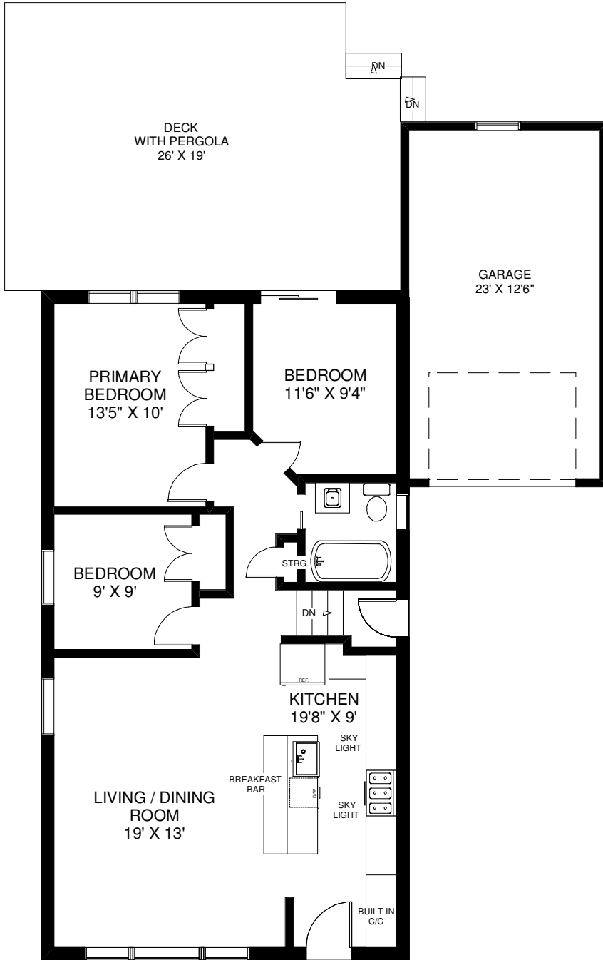
MAIN FLOOR
