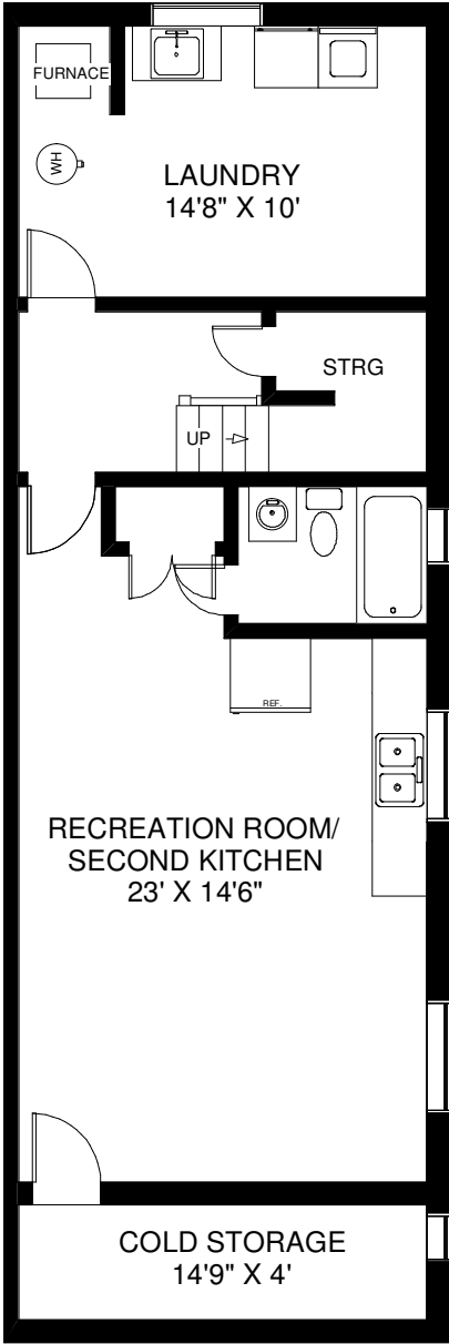
LOWER FLOOR
