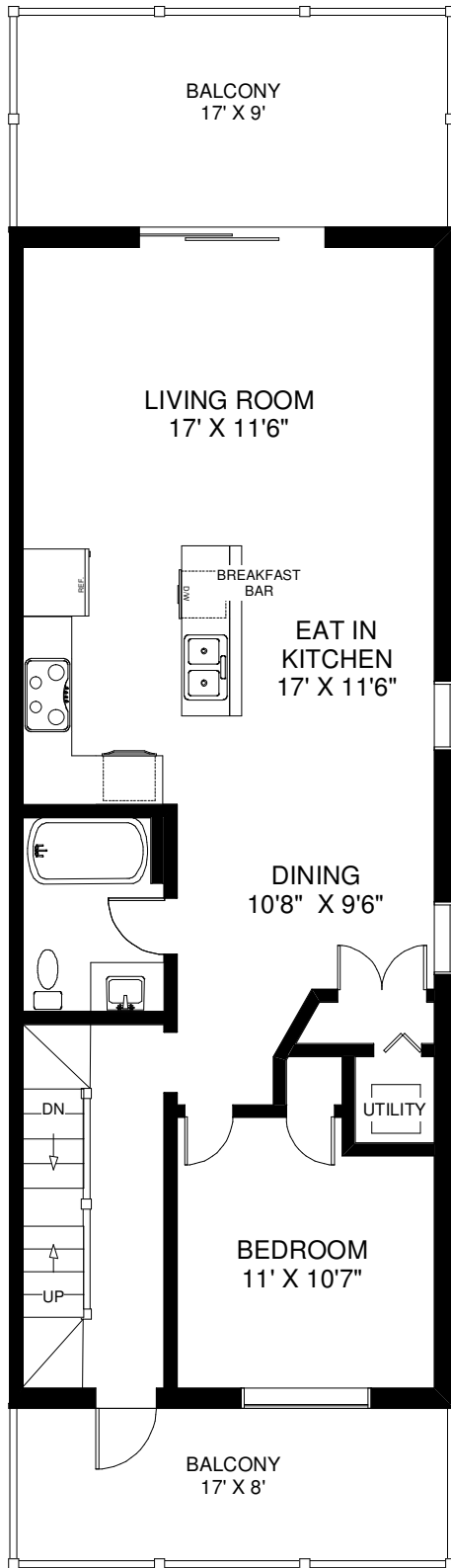
CEILING HT 8' SECOND FLOOR
